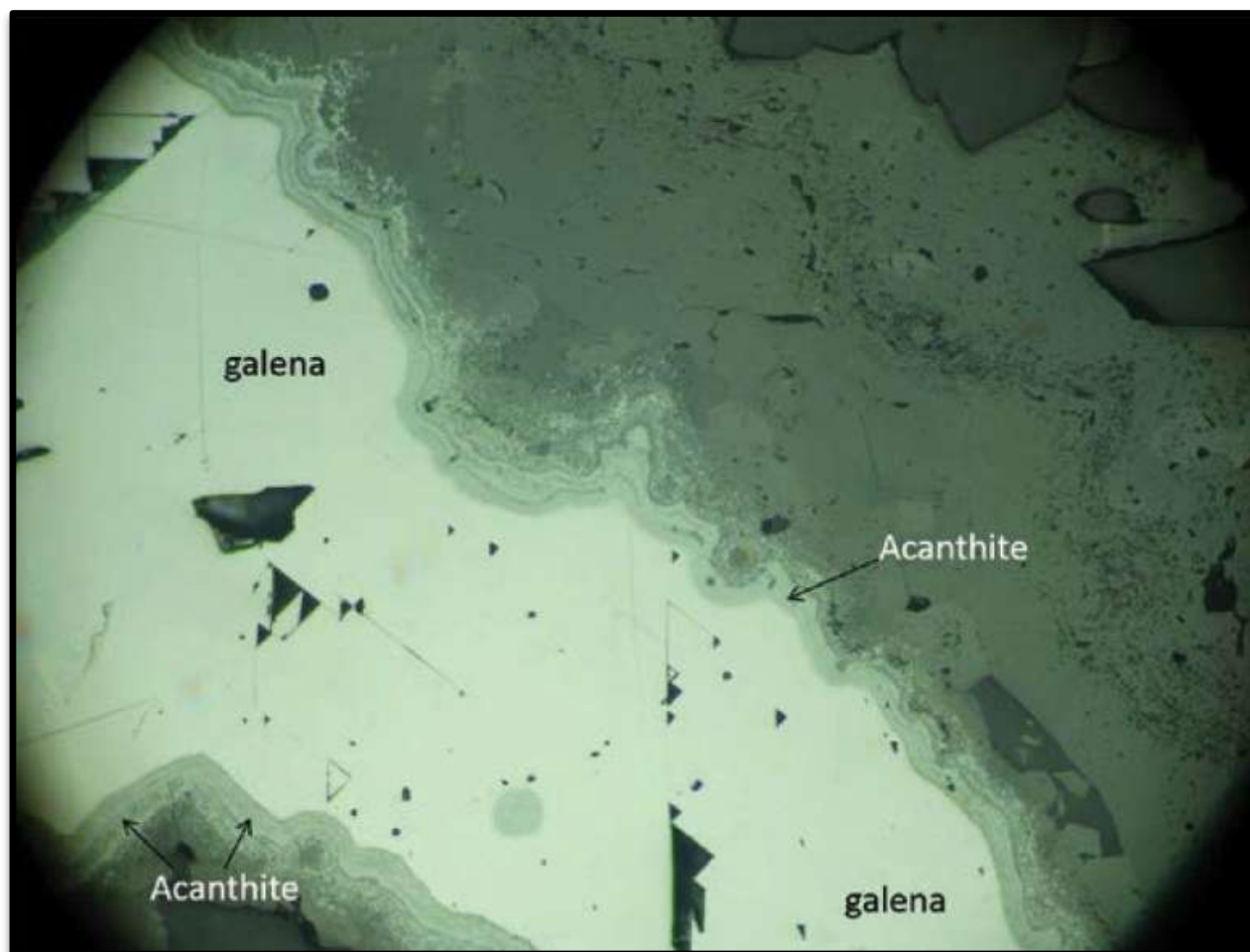
Figure 14: A reflected light microscopy image of mineralization from the Alice mine (Acanthite (Ag 2 S) and Galena (PbS)) (Gammons et al, 2016).
